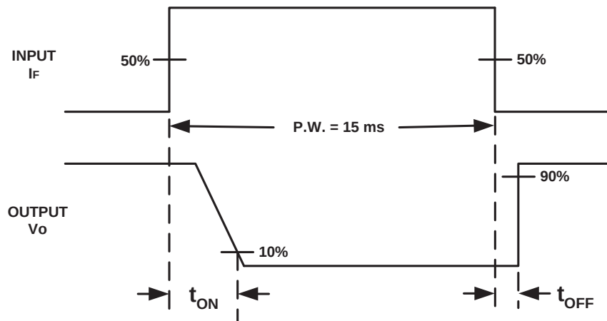
Figure 15. Switching Test circuit for t ON , t OFF
