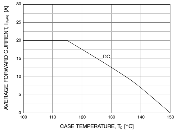
Figure 8. Forward Current Derating Curve
