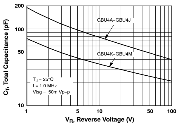
Figure 5. Total Capacitance
