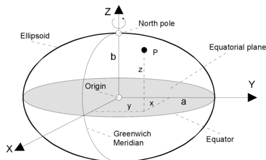
Figure 5: Earth-Centered Earth-Fixed Coordinate System
