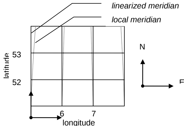
Figure 7: Spatial Distortion as Result of Mapping Ellipsoidal Coordinates to Local Tangent Plane (LTP)
