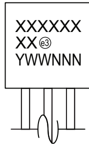
3-lead SOT-23
