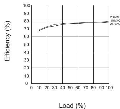
RAC04-0512DC/277
