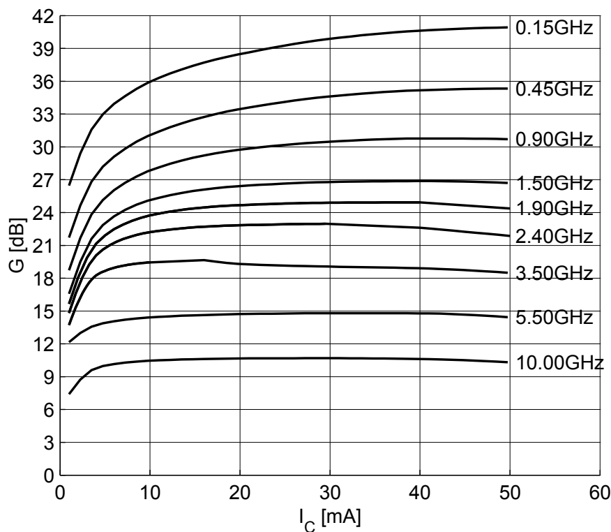
Figure 12 Maximum power gain G_{\text{max}} = f(I_C) , V_{CE} = 3 \text{ V} , f = \text{parameter in GHz}
