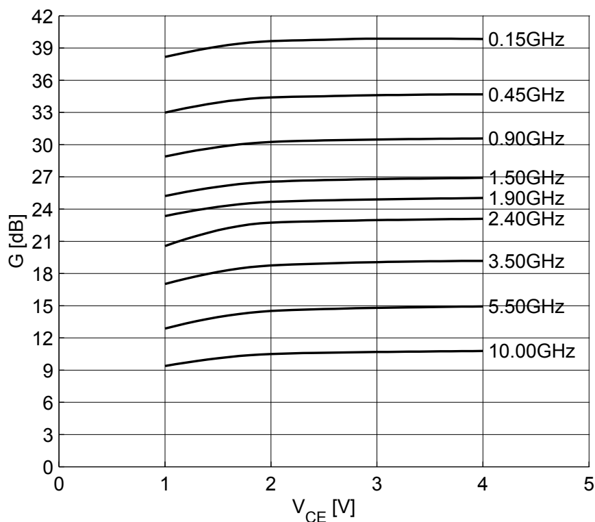
Figure 13 Maximum power gain G_{\text{max}} = f(V_{CE}) , I_C = 30 \text{ mA} , f = \text{parameter in GHz}
