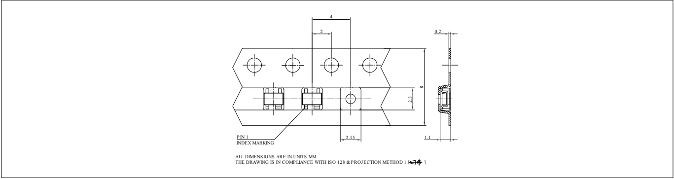
Figure 23 Tape dimensions
