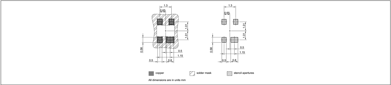
Figure 21 Foot print
