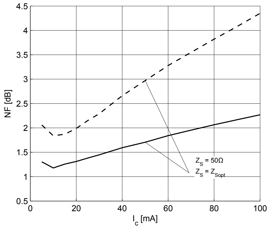
Figure 20 Noise figure NF_{50} = f(I_C) , Z_S = 50 \Omega , NF_{min} = f(I_C) , Z_S = Z_{S,opt} , V_{CE} = 3 V , f = 1.9 GHz
