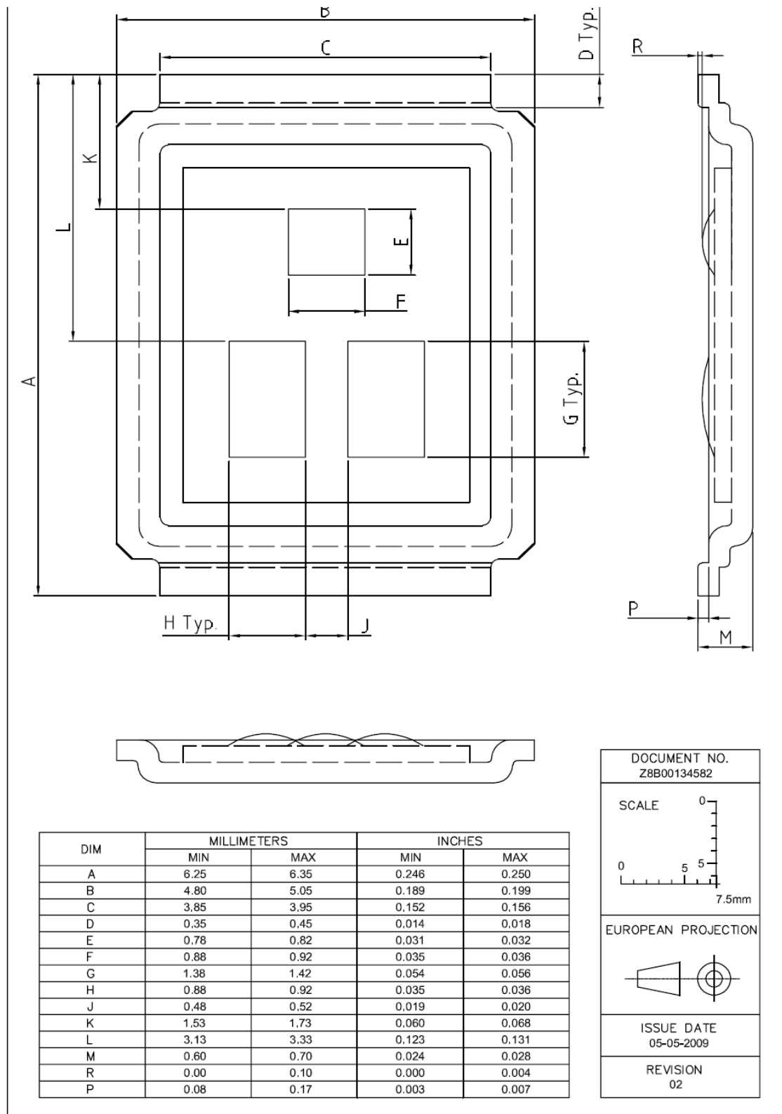
Figure 1 Outlines MG-WDSN-2, dimensions in mm/inches
