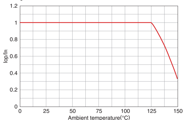
Derating
