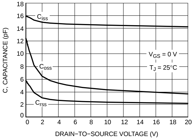
Figure 16. Capacitance Variation
