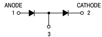
BAV99WT1 SC-70, CASE 419, STYLE 9
