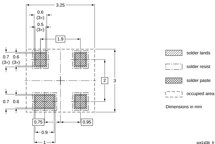
Fig 11. Reflow soldering footprint SOT143B
