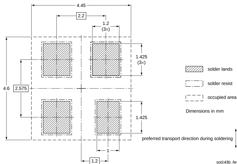
Fig 12. Wave soldering footprint SOT143B
