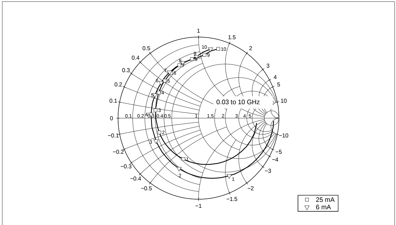
Figure 5-13 Input Matching S_{11} = f(f) , V_{CE} = 3 V, I_C = 6 / 25 mA
