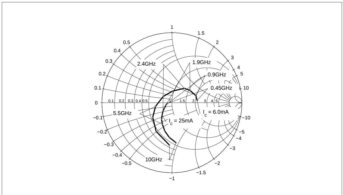
Figure 5-14 Source Impedance for Minimum Noise Figure Z_{opt} = f(f) , V_{CE} = 3 V, I_C = 6 / 25 mA
