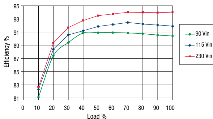
MVAC250-12F Efficiency
