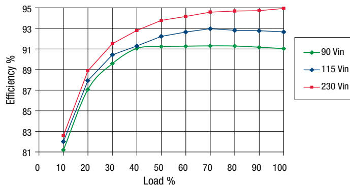
MVAC250-48F Efficiency
