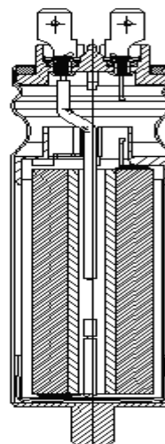
In order to allow a correct working of the safety device and to assure a sufficient electric insulation, a room of almost 10 mm will have to be assured.
