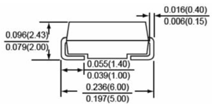
SMB/DO-214AA
