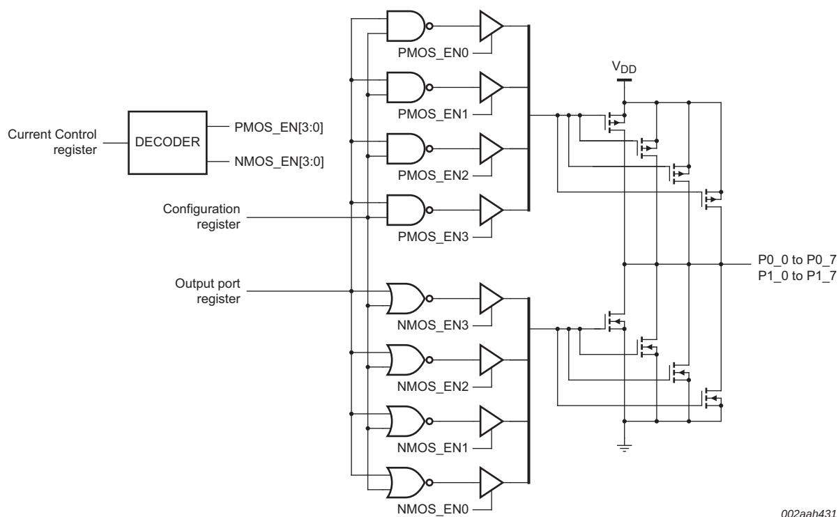
Fig 16. Simplified output stage
