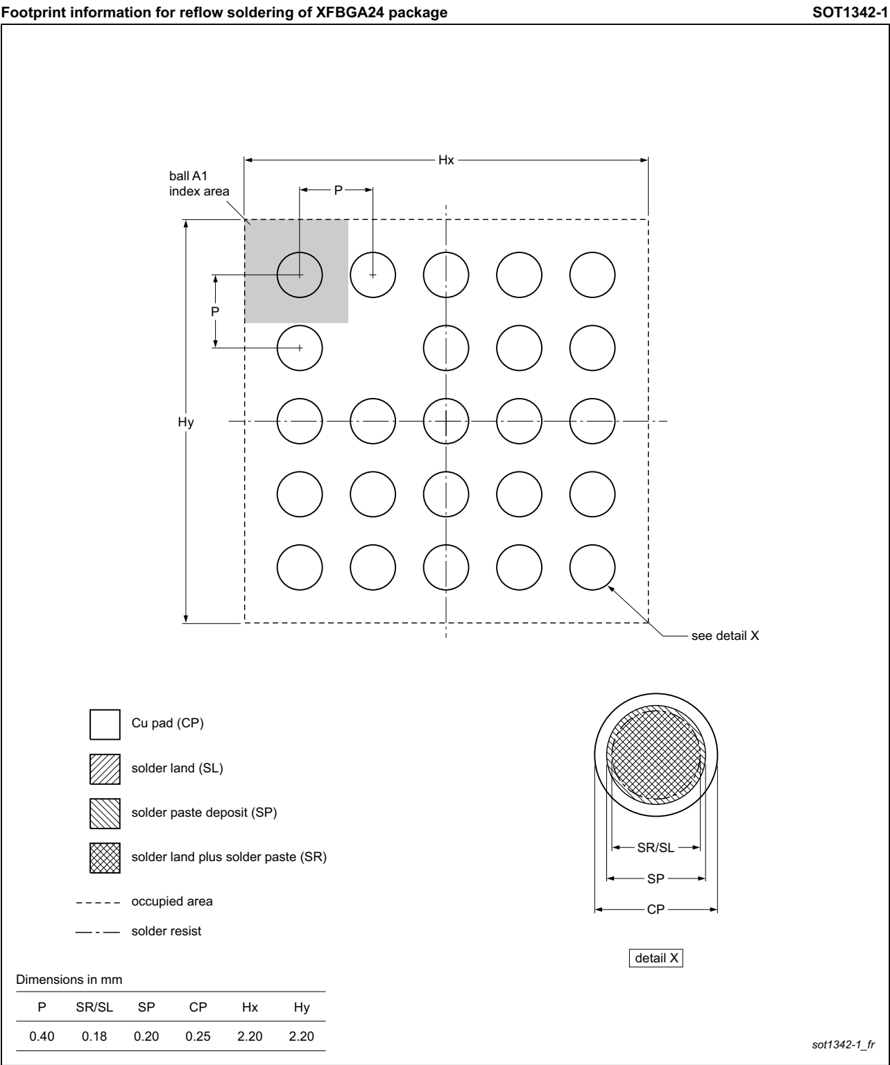
Fig 47. PCB footprint for SOT1342-1 (XFBGA24); reflow soldering
