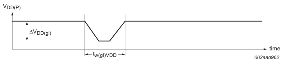
Fig 21. Glitch width and glitch height
