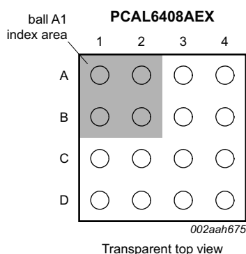
Fig 5. Pin configuration for 1.6 mm × 1.6 mm XFBGA16
