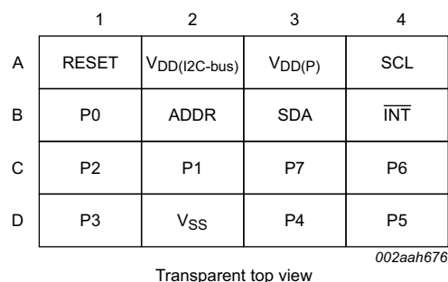
Fig 6. Ball mapping for 1.6 mm × 1.6 mm XFBGA16
