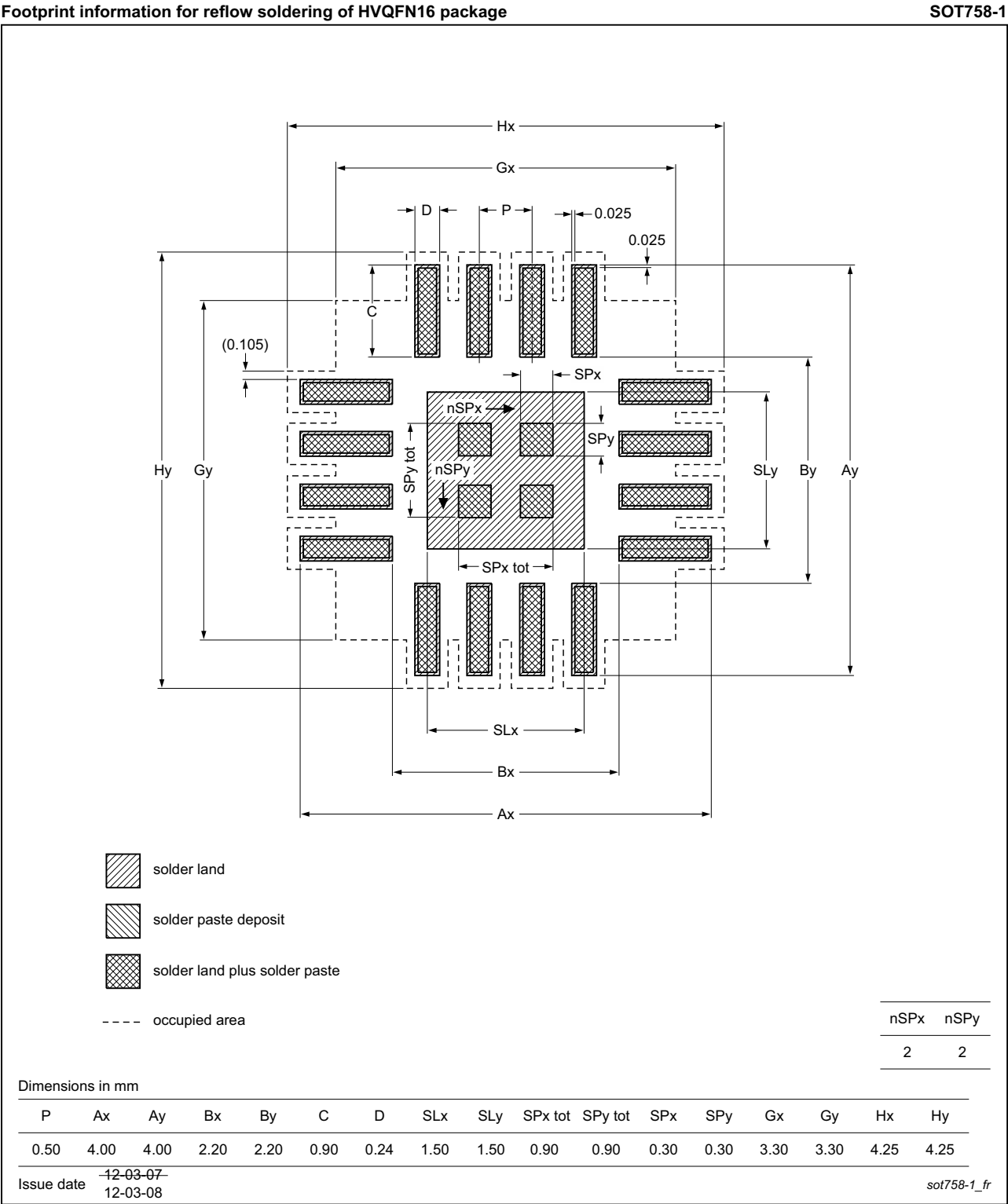
Fig 40. PCB footprint for SOT758-1 (HVQFN16); reflow soldering
