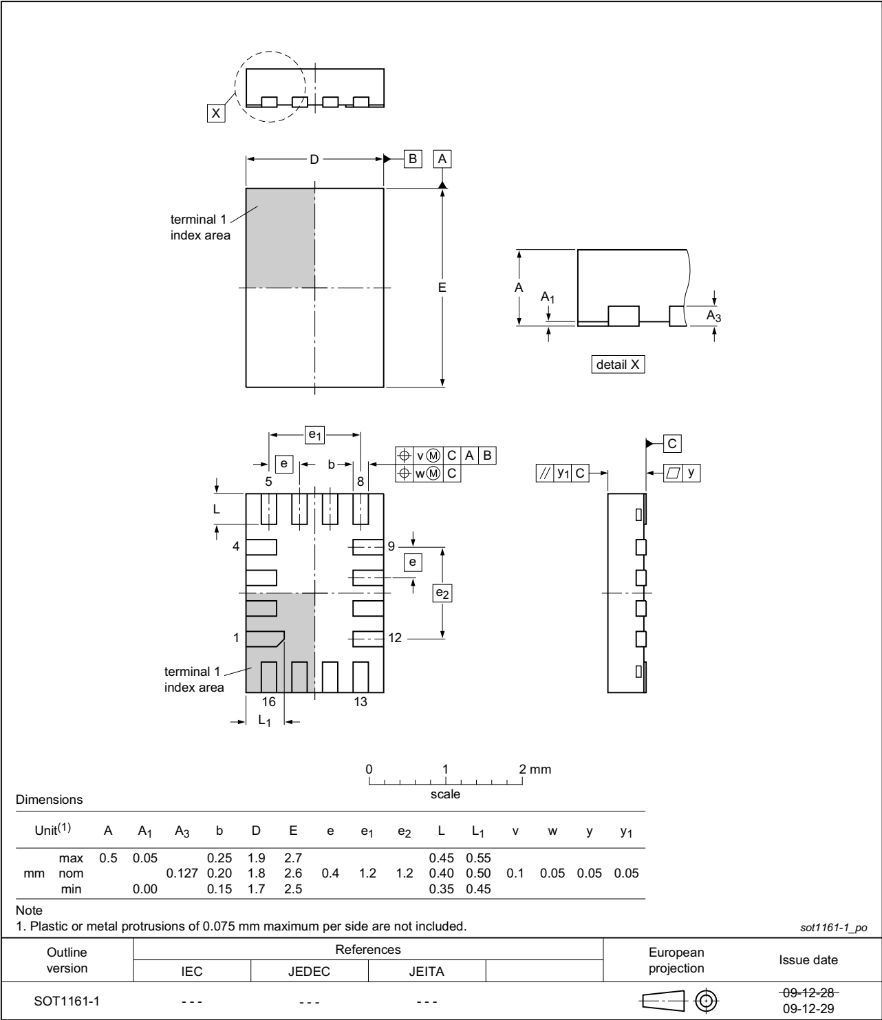
Fig 37. Package outline SOT1161-1 (XQFN16)
