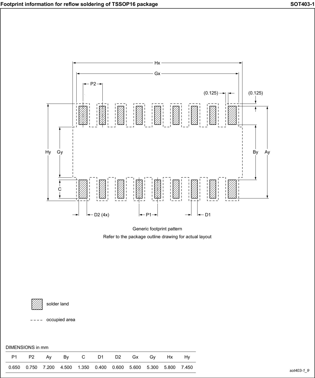
Fig 41. PCB footprint for SOT403-1 (TSSOP16); reflow soldering
