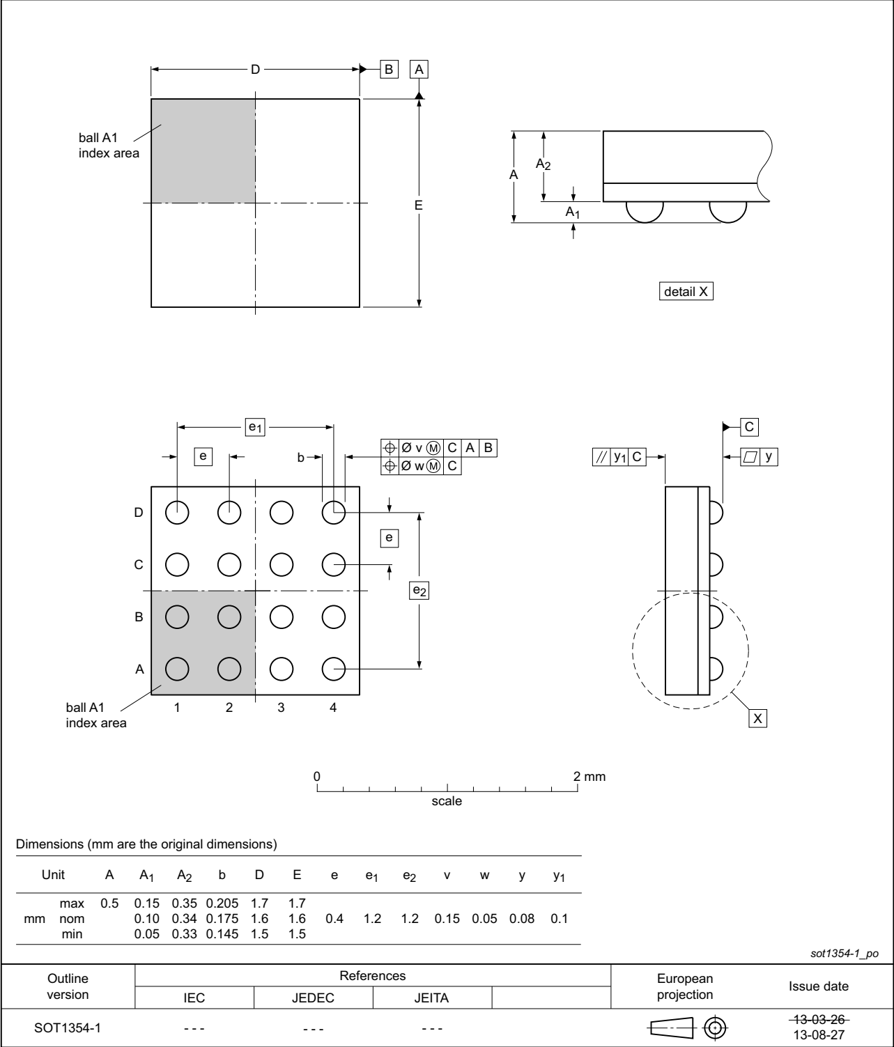
Fig 38. Package outline SOT1354-1 (XFBGA16)
