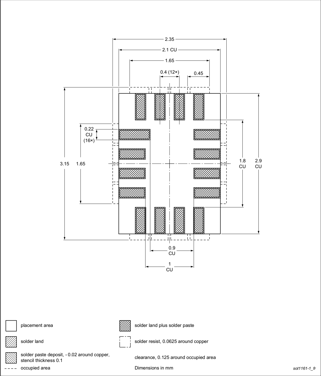
Fig 42. PCB footprint for SOT1161-1 (XQFN16); reflow soldering
