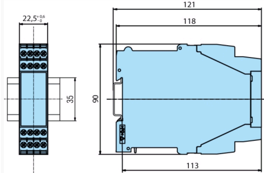
KNE3-YS - Screw terminals
