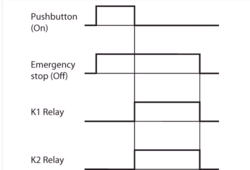
Function diagram
