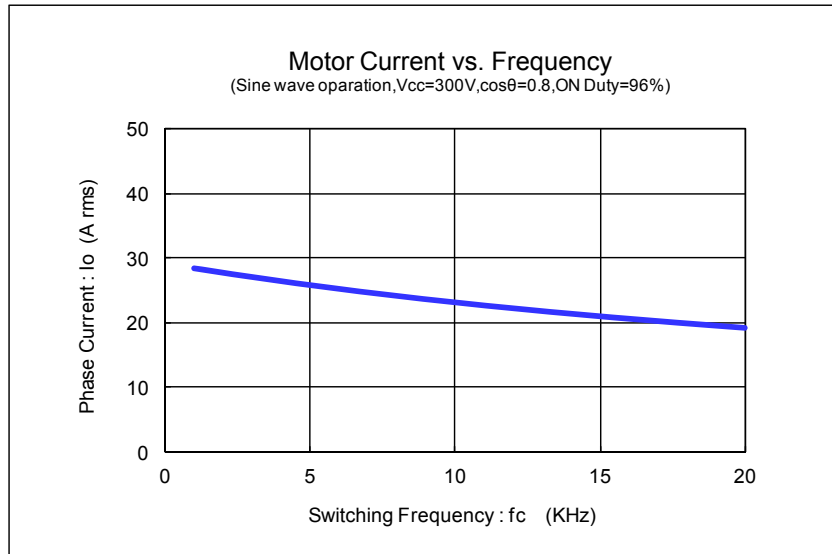
Fig.12 Maximum sinusoidal phase current as function of switching frequency. at T_c=100^\circ\text{C} , V_{cc}=300V
