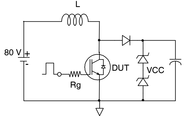
Fig.C.T.2 - RBSOA Circuit
