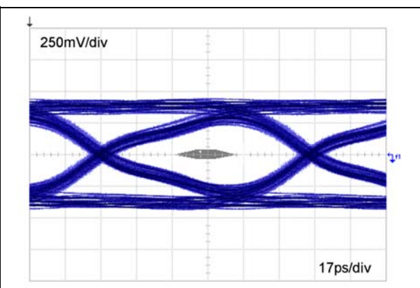
Figure 18. USB3.1 (10 Gbps) eye diagram with device
