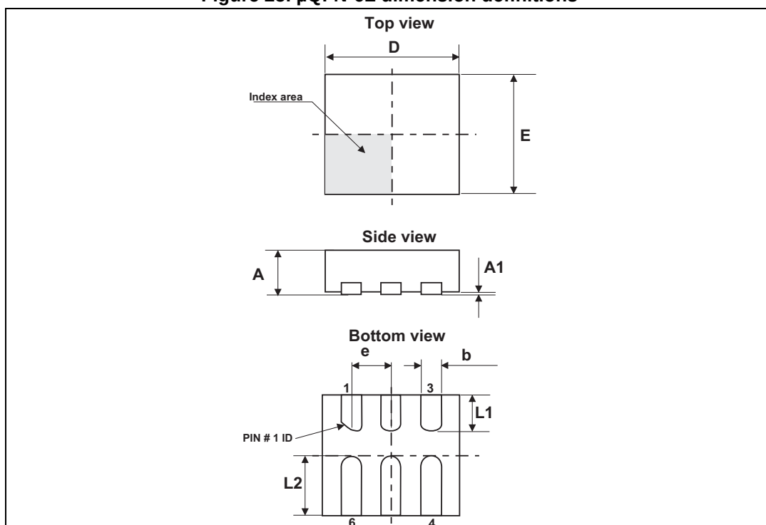
Figure 25. \mu QFN-6L dimension definitions
