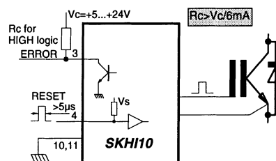
Fig.5 Driver status information ERROR, and RESET
