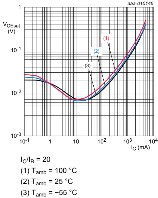
Fig. 8. Collector-emitter saturation resistance as a function of collector current; typical values
