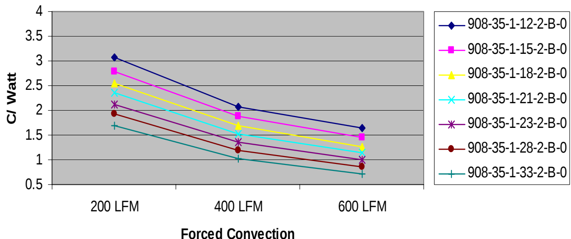
Thermal Performance
