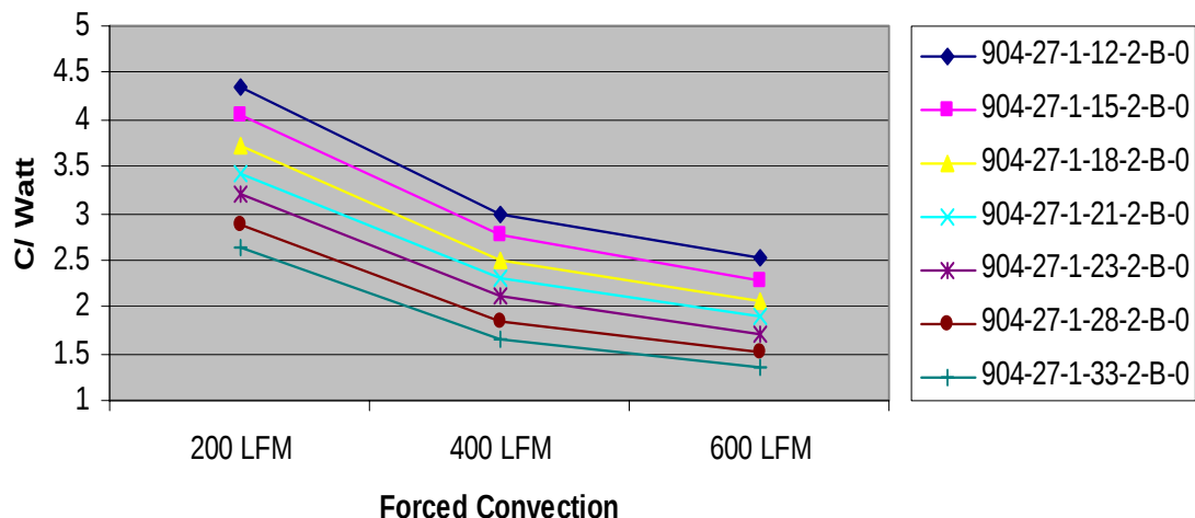
Thermal Performance
