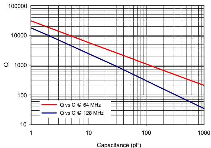
S42E Q vs. Capacitance, Typical
