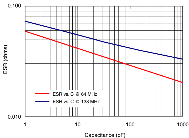
S42E ESR vs. Capacitance, Typical
