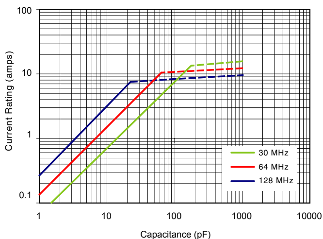
Current Rating vs. Capacitance, S42E, Typical (Preliminary)
