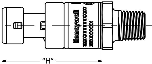
Figure 7. Connector Dimensions (For reference only: mm/[in].)
