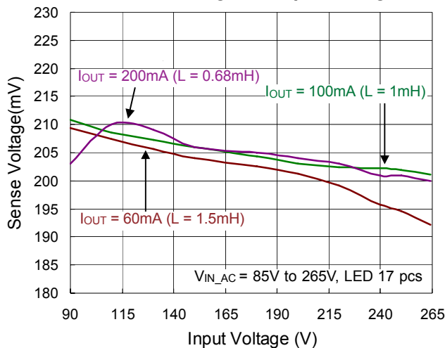
Sense Voltage vs. Input Voltage
