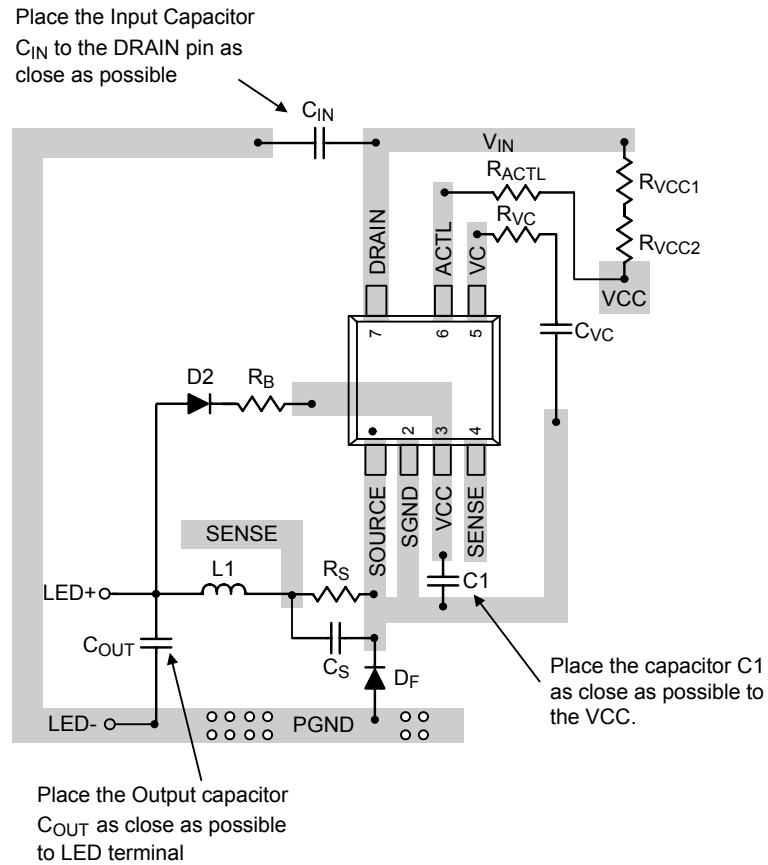
Figure 2. PCB Layout Guide
