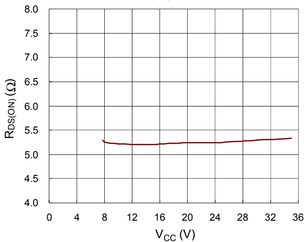
R_{DS(ON)} vs. V_{CC}
