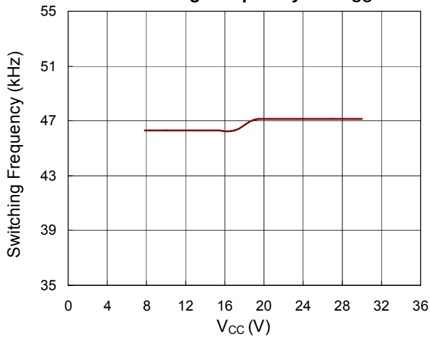
Switching Frequency vs. V_{CC}
