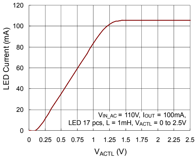
LED Current vs. V_{ACTL}
