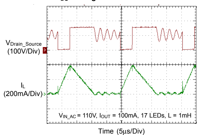
V_{DS} Voltage and Inductor Current
