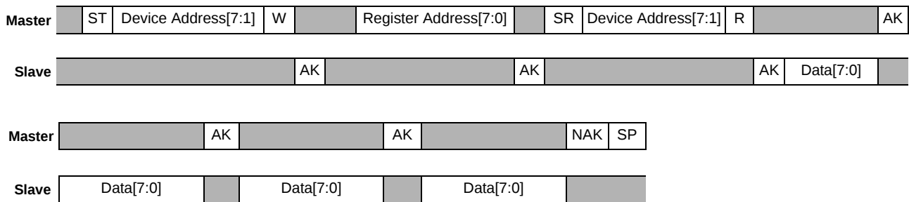
Figure 11. Multiple Byte Read timing (I²C)
