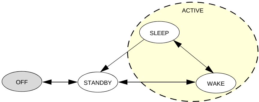
Figure 5. Operating modes for MMA8652FC
