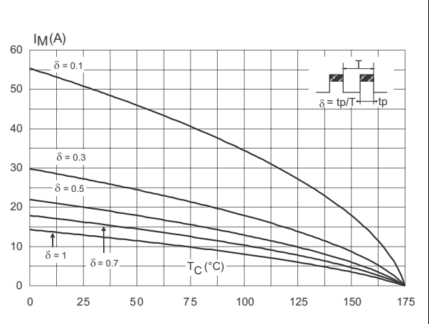
Figure 4. Peak forward current versus case temperature (per diode)
