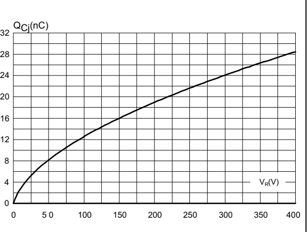
Figure 8. Total capacitive charges versus reverse voltage applied (typical values, per diode)
