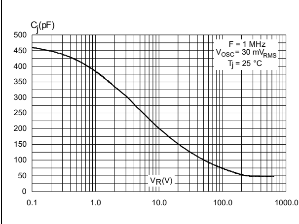
Figure 5. Junction capacitance versus reverse voltage applied (typical values, per diode)
