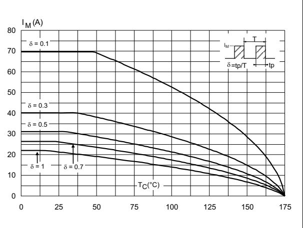
Figure 4. Peak forward current versus case temperature (TO-220AC, DPAK, D²PAK)
