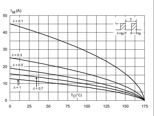
Figure 4. Peak forward current versus case temperature (TO-220AC and DPAK)
