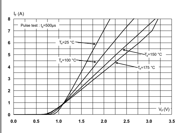
Figure 1. Forward voltage drop versus forward current (typical values, low level)
