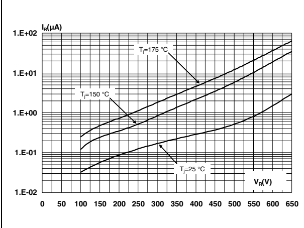
Figure 3. Reverse leakage current versus reverse voltage applied (typical values)
