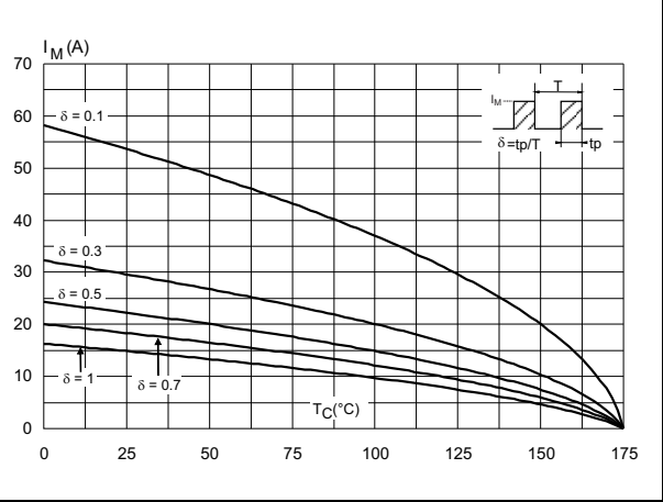
Figure 4. Peak forward current versus case temperature (TO-220AC, DPAK, D 2 PAK)
