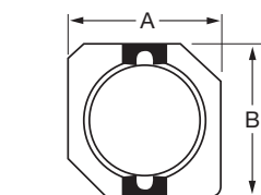
Recommended Solder PAD Layout
