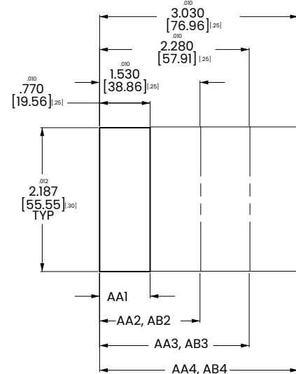
PANEL CUTOUT DETAIL
