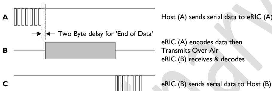
Figure 5 Timing Diagram
