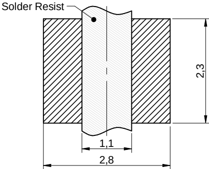
No vias and traces in restricted area Scale - 12:1
