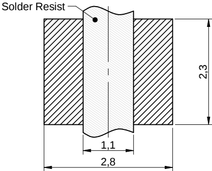
No vias and traces in restricted area Scale - 13:1
