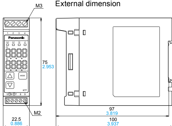
External dimension
