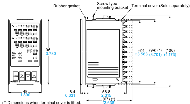
External dimension
