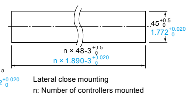
When installing in series
