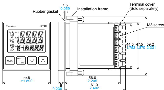
External dimension
