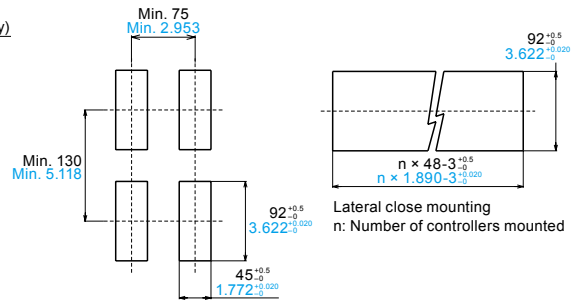
Panel cutout
