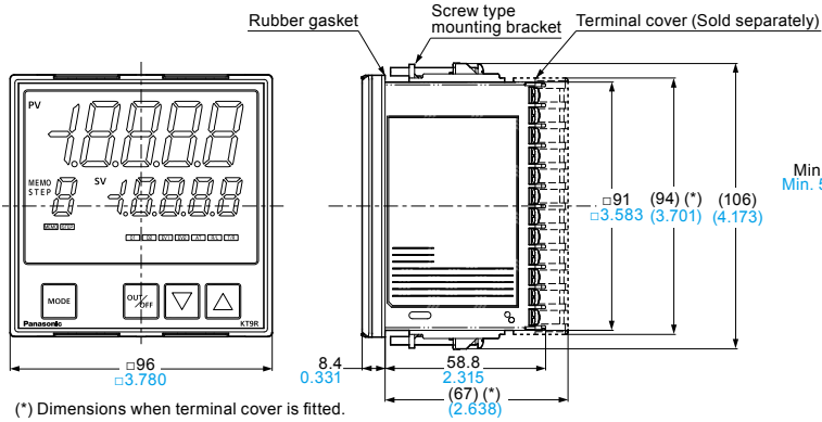
External dimension
