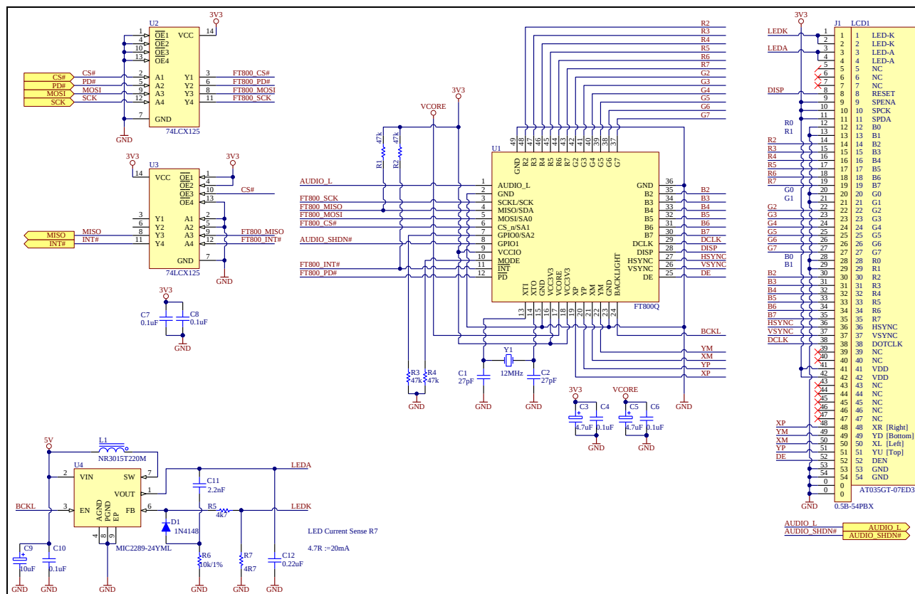
Figure 4-1 - VM800B35A (3.5" Version)
