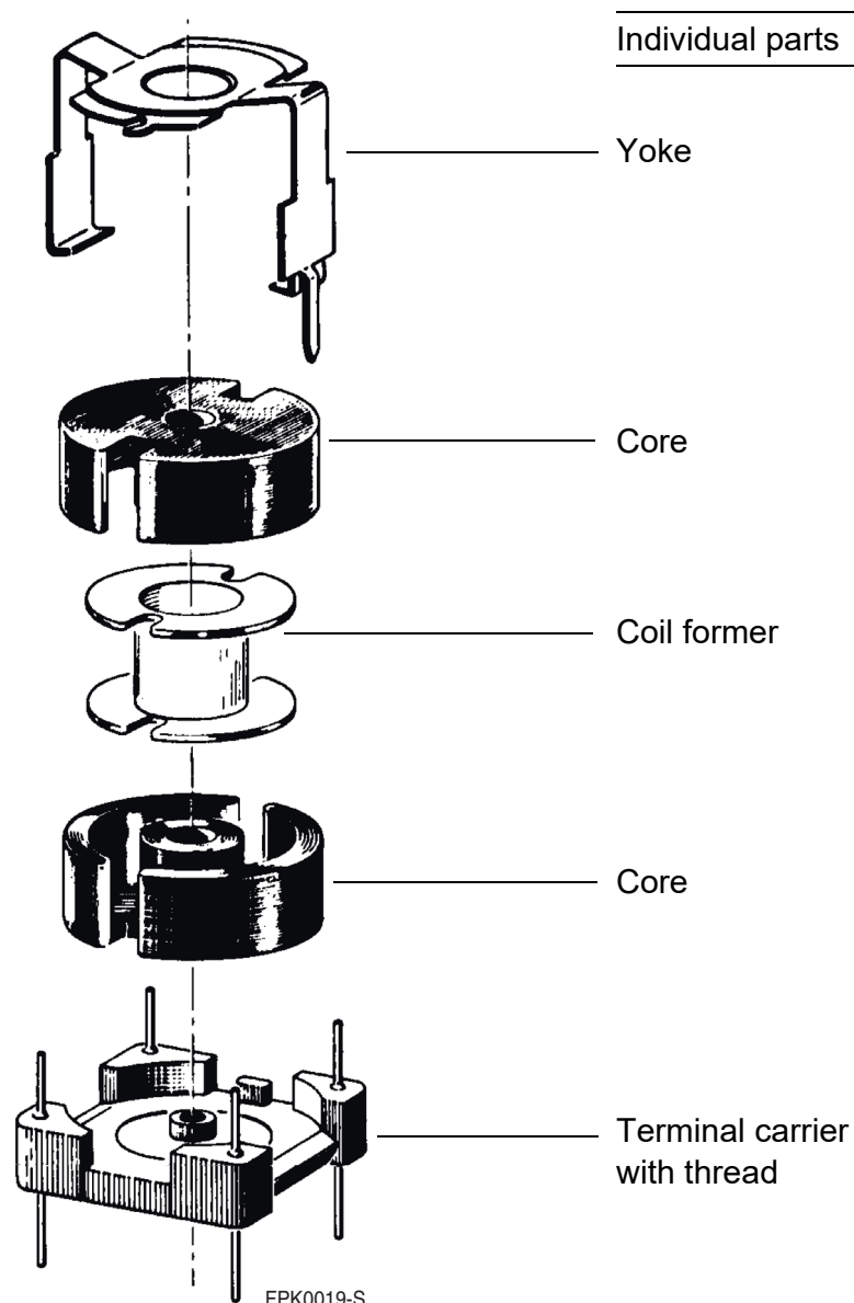
Example of an assembly set for printed circuit boards
