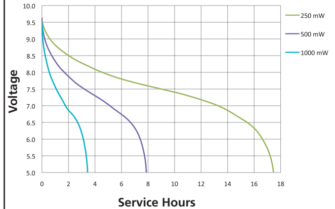
Ultra Power 9V Constant Power
