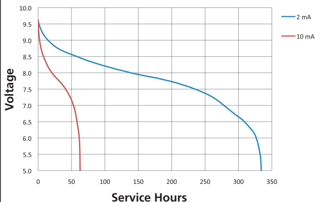
Ultra Power 9V Constant Current
