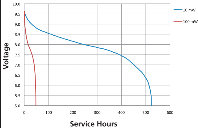
Ultra Power 9V Constant Power
