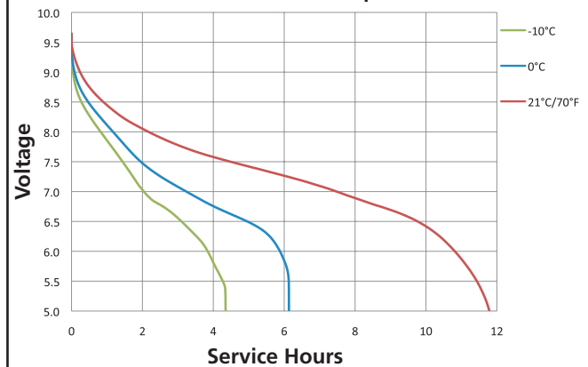
Ultra Power 9V Constant Temperature at 50 mA
