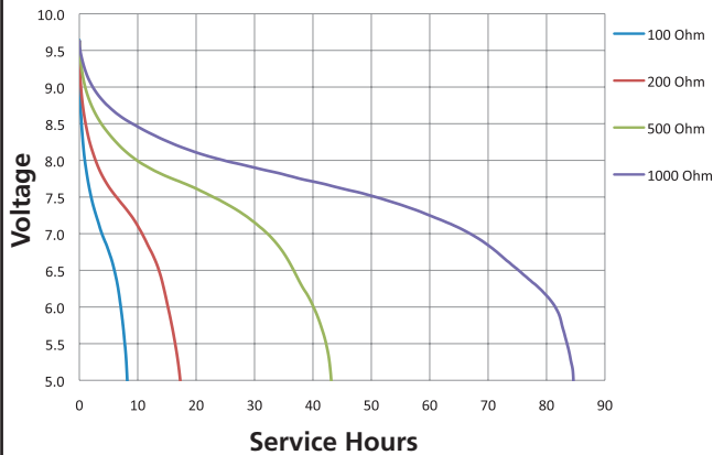
Ultra Power 9V Constant Resistance
