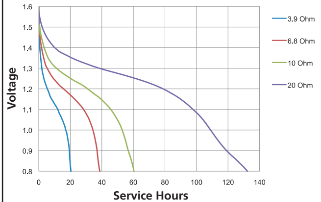
Plus Power C Constant Resistance
