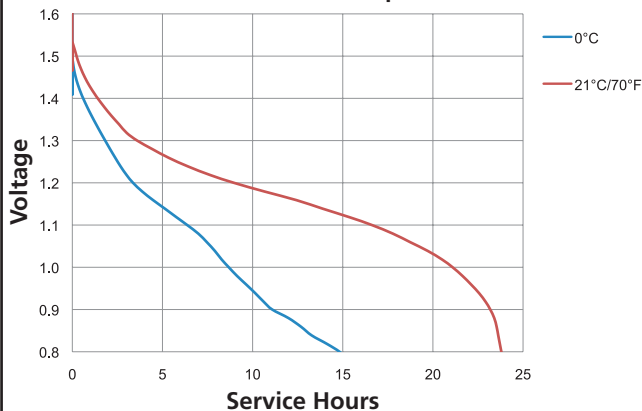
Plus Power C Constant Temperature at 250 mA
