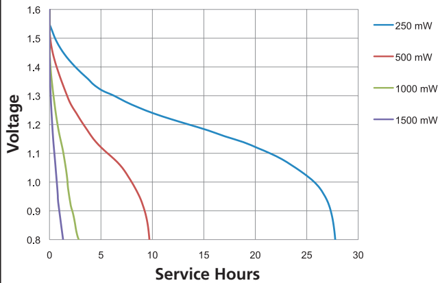
Plus Power C Constant Power
