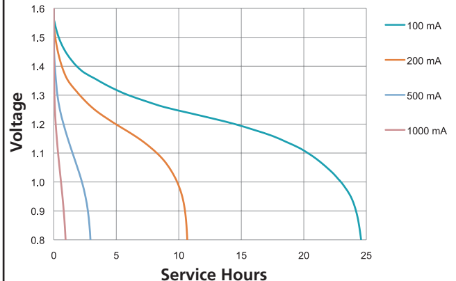
Plus Power AA Constant Current
