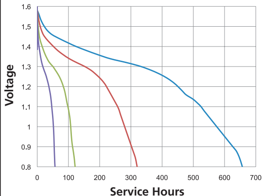
Plus Power AA Constant Current
