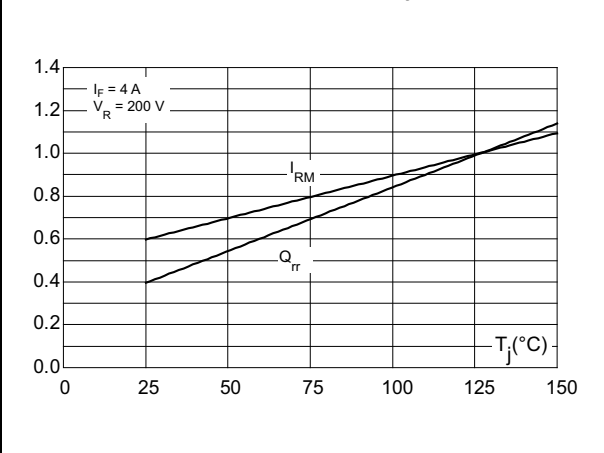
Figure 7. Dynamic parameters versus junction temperature (reference: T_j = 125\text{ }^{\circ}\text{C} )
