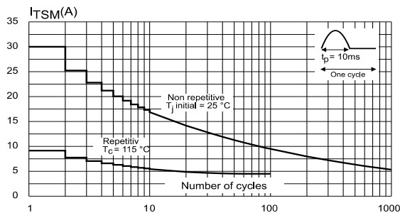
Figure 9: Surge peak on-state current versus number of cycles
